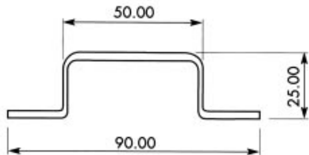
Section No. G481, 0.881 kg/m, per 263
