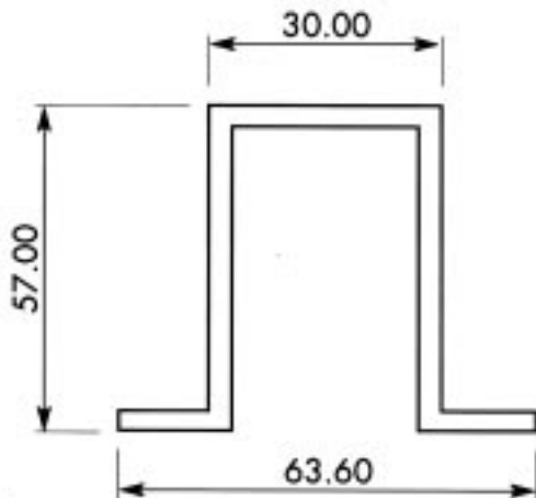
Section No. 5081, 1.798 kg/m, per 358
