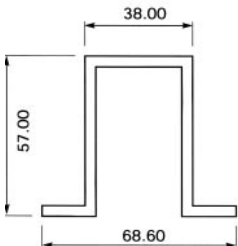
Section No. 5081, 1.796 kg/m
