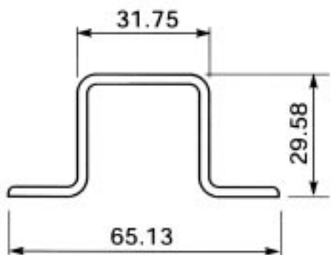
Section No. X538, 0.723 kg/m
