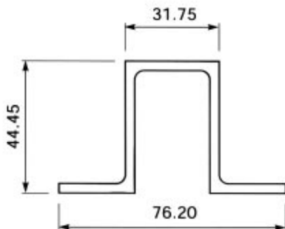
Section No. 0644, 1.396 kg/m
