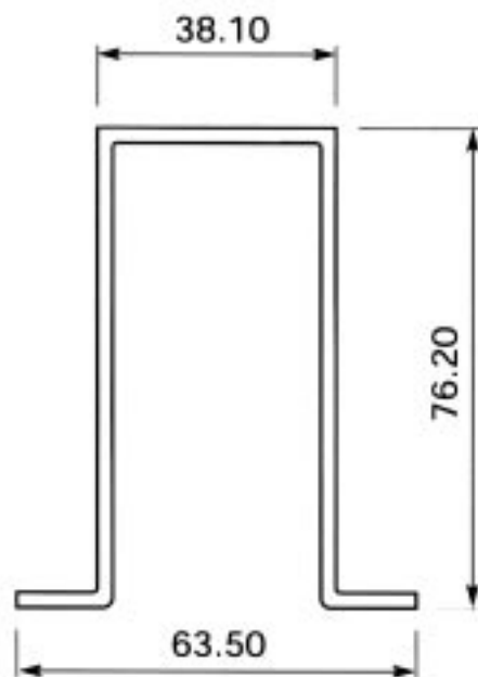
Section No. 2418, 1.375 kg/m
