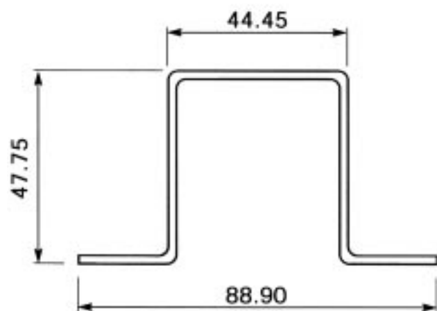
Section No. 0954, 0.997 kg/m
