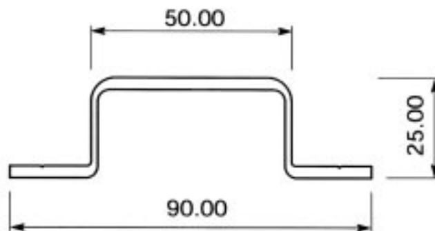
Section No. G481, 0.881 kg/m
