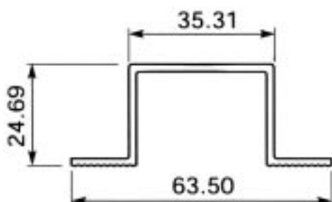
Section No. 2184, 0.517 kg/m
