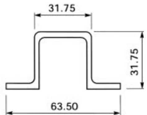
Section No. Z741, 0.952 kg/m
