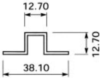
Section No. 4519, 0.256 kg/m
