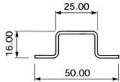
Section No. 0582, 0.332 kg/m
