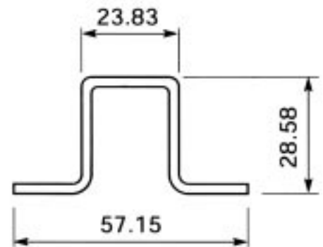
Section No. 0297, 0.738 kg/m
