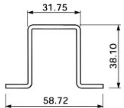
Section No. 0866, 0.812 kg/m
