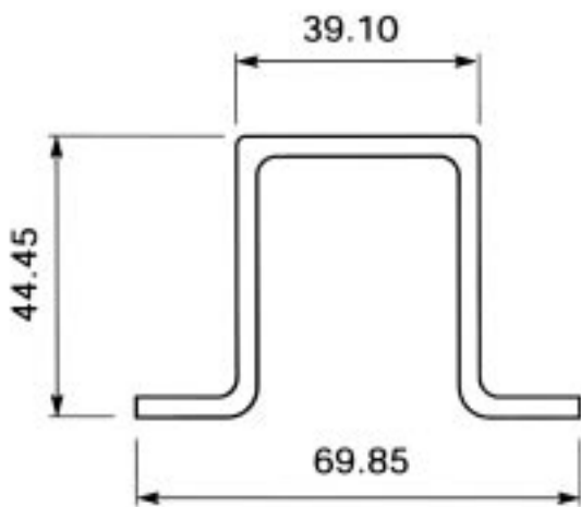
Section No. 0296, 1.360 kg/m
