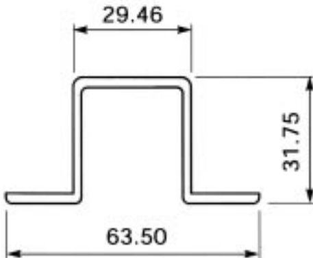
Section No. 0577, 0.751 kg/m
