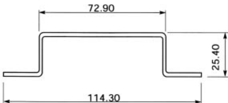
Section No. 7205, 0.902 kg/m
