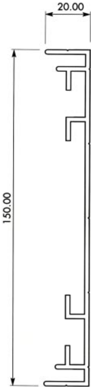
Section No. X540, 1.418 kg/m per 529
