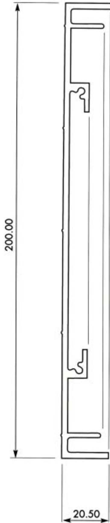
Section No. J277, 2.033 kg/m per 614
