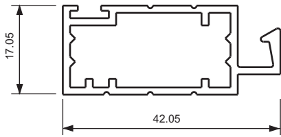
Section No. 9775 Flyscreen Door Frame 5m Lengths
