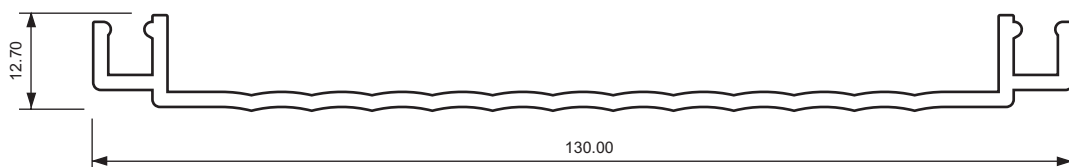
Section No. 7675, Push Plate
