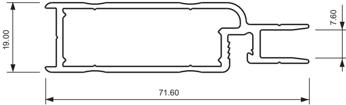
Section No. Z785 Security Door Frame
