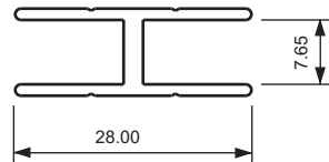
Section No. X574
