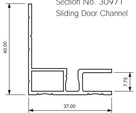
Section No. 6179 Security Window Frame with Leg
