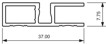
Section No. 5663 Security Window Frame
