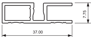
Section No. F9294
