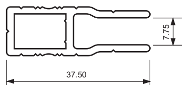
Section No. G253 Heavy Duty Window Frame
