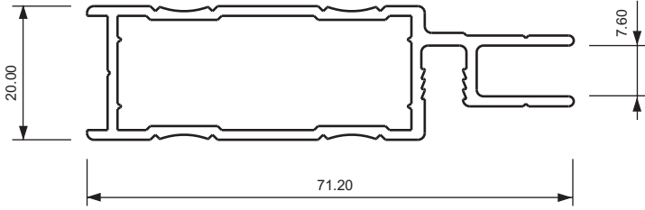
Section No. Z785 Security Door Frame
