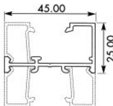
Section No. J349 Glazing Frame 0.466 kg/m per 216
