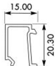
Section No. J350 Square Bead 0.193 kg/m per 117
