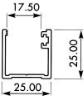
Section No. E770, 0.347 kg/m per 168
