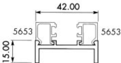
Section No. 5620 Infill Vision Rail 0.484 kg/m, per 157
