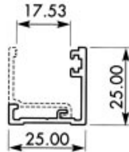
Section No. E772, 0.284 kg/m per 140
