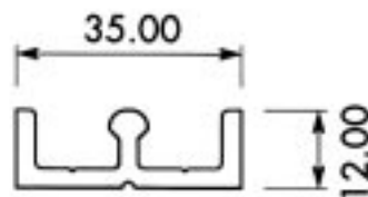
Section No. 6350 Door Track 0.518 kg/m, per 127
