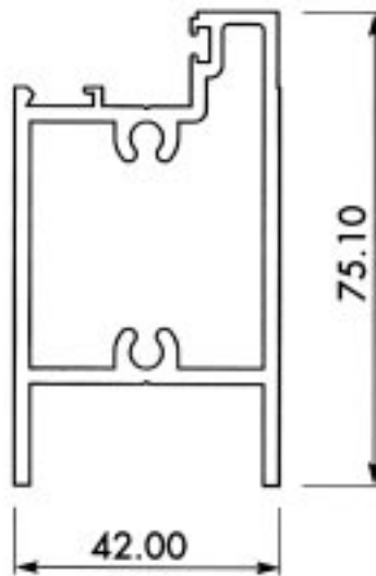
Section No. 8163 Top Rail 1.732 kg/m, per 292
