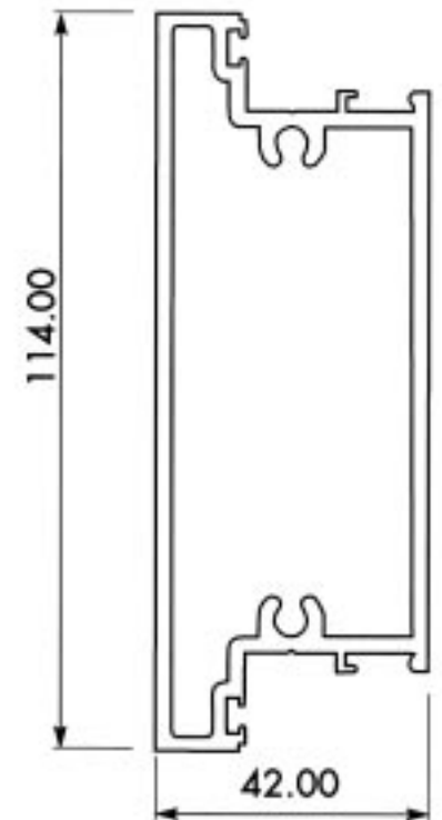
Section No. 8165 Wide Vision Rail 2.285 kg/m, per 363
