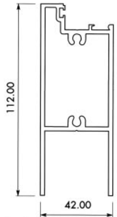
Section No. 8164 Bottom/Top Rail 2.232 kg/m, per 410
